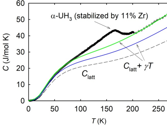
Fig. 1. Temperature dependence of specific heat of \alpha\text{-UH}_3 , the calculated bare lattice part and lattice and electronic part for different \gamma . The maximum at T = 170 K is the magnetic phase transition.
