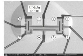
Fig. 3. SEM image of a microdevice of \text{U}_2\text{Ni}_2\text{Sn}
