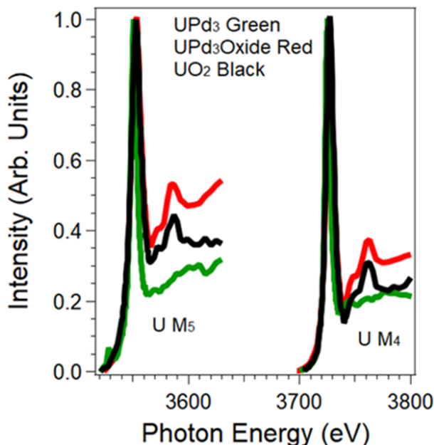
Figure 1. Shown here are the UM_4 and UM_5 Total Fluorescence Yield (TFY) measurements for UO_2 (black), cast UPd_3 (green) and oxide contaminated UPd_3 (red). All of the spectra were normalized to unity. Note the signature peak of the oxide near h\nu = 3580\text{ eV} and h\nu = 3760\text{ eV} .
