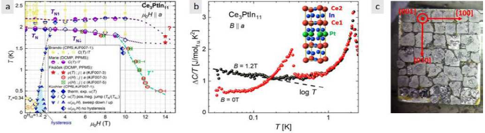
Figure 1: The H - T phase diagram of \text{Ce}_3\text{PtIn}_{11} for \mu_0 H \parallel a . Data were collected from specific heat, thermal expansion, magnetostriction, resistivity, and magnetoresistance experiments. Lines are a guide to the eyes. (b) The zero field specific heat and in an applied field of \mu_0 H = 1.2 \text{ T} \geq \mu_0 H_{c2} after subtracting the nuclear contribution arising from In. The \log T -dependence points to the presence of quantum critical fluctuations of a nearby QCP. The inset shows the \text{Ce}_3\text{PtIn}_{11} unit cell. (c) Sample mosaic used for \mu\text{SR} experiment. It consists of 36 co-aligned single crystals ( m_{\text{total}} \approx 150 \text{ mg} ) and covers an area of 4.5 \times 5 \text{ mm}^2 .
