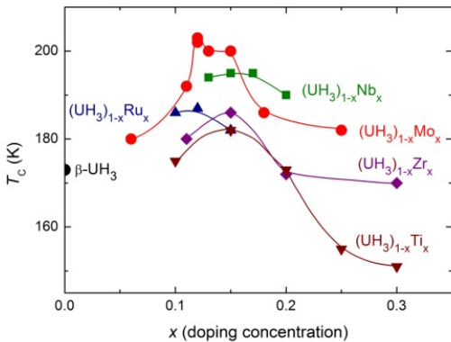
Fig. 2. T-concentration dependence of the Curie temperature of the (\text{UH}_3)_{1-x}\text{T}_x hydrides. The lines are for guiding the eyes.
