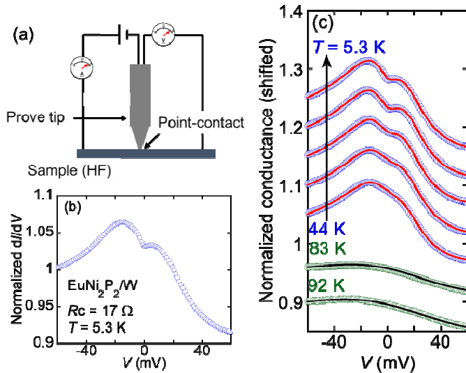
Fig 1. (a) The schematic diagram of PCS measurement. (b) The dI/dV spectra of \text{EuNi}_2\text{P}_2 with W probe tip. (c) Temperature dependence of dI/dV spectra. The symbols correspond to the experimental data. Black and red solid line correspond to the theoretical calculation using Fano model and MDC model, respectively.
