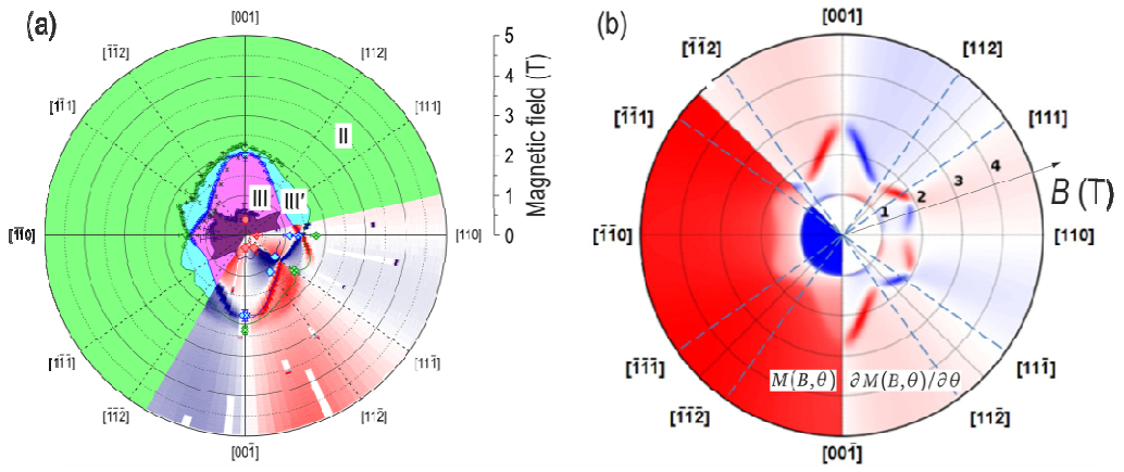
Fig. 1. (a) Field-angular magnetic phase diagram of \text{CeB}_6 measured using torque magnetometry. (b) Angle derivative of the magnetization, calculated ab initio for a two-site model.
