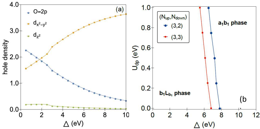
Fig. 1. For increasing \Delta in the periodic \text{Ni}_4\text{O}_8 cluster: (a) hole densities as obtained for the undoped cluster with N(\text{up})=N(\text{down})=2 holes, and (b) phase diagram for doped cluster with (3,2) or (3,3) holes in the \{\Delta, U_{dp}\} plane. Lines in (a) show the hole number in \text{Ni}(x^2-y^2) orbitals (orange), in \text{O}(2p) orbitals (blue), and in \text{Ni}(z^2) orbitals (green). Other parameters (all in eV): t_{pd}=1.3 , t_{pp}=0.55 , U_d=8.34 , J_d=1.18 , U_p=4.4 , J_p=0.8 .
