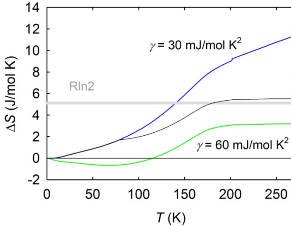
Fig. 2. Related changes of entropy \Delta S(T) counted from T = 0 . It compares the entropy including the change of electronic part at T = 80 K (green) with purely magnetic one (black).
